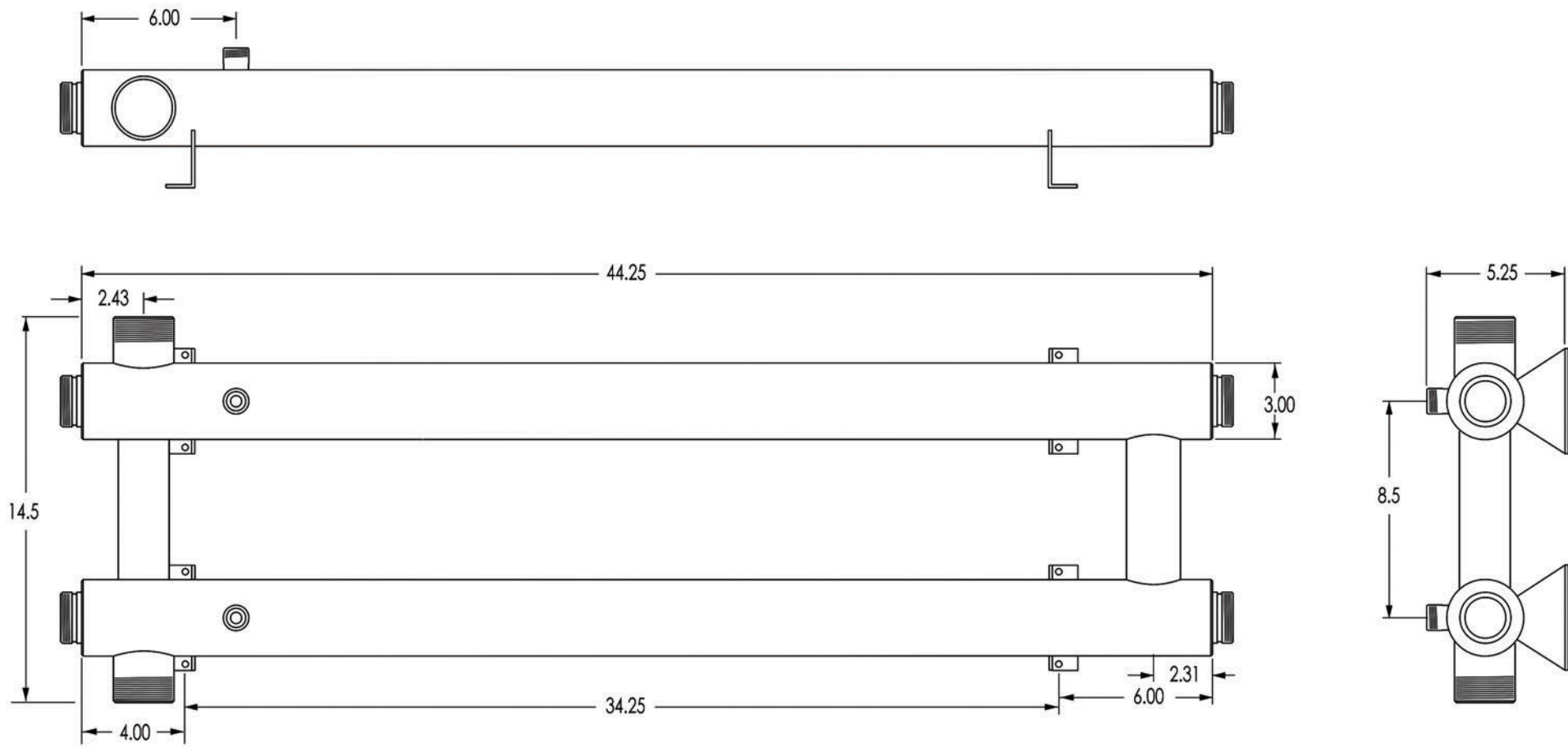
Wyckomar Inc. UV-6000 All measurements in inches (1" = 25.4 mm)
